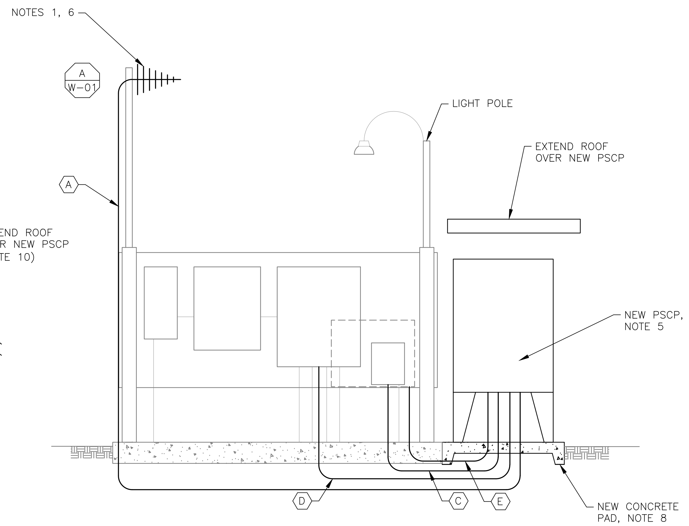
3 NEW SCADA PANEL ELEVATION SCALE: NOT TO SCALE
