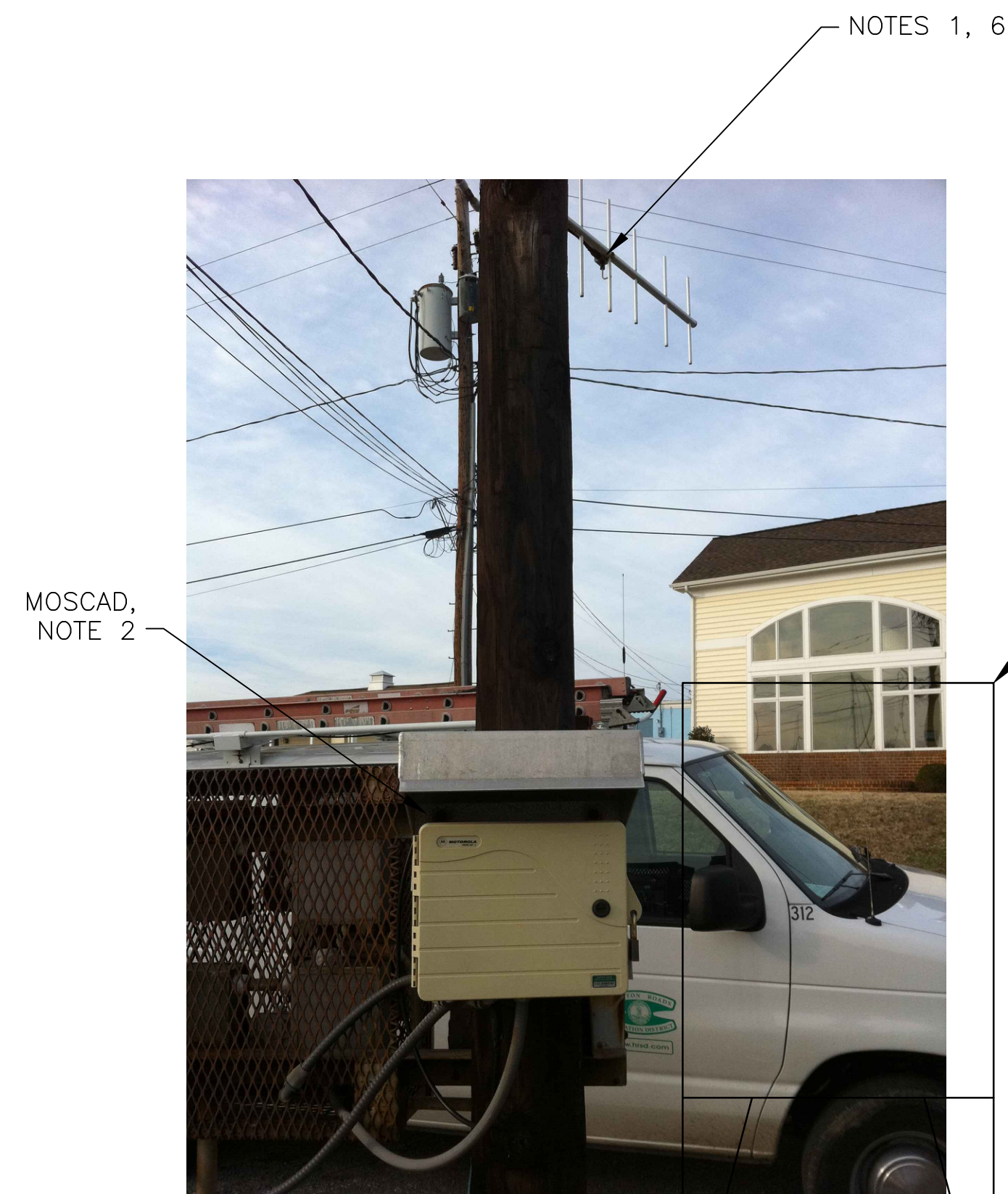
2 ANTENNA LOCATION SCALE: NOT TO SCALE
