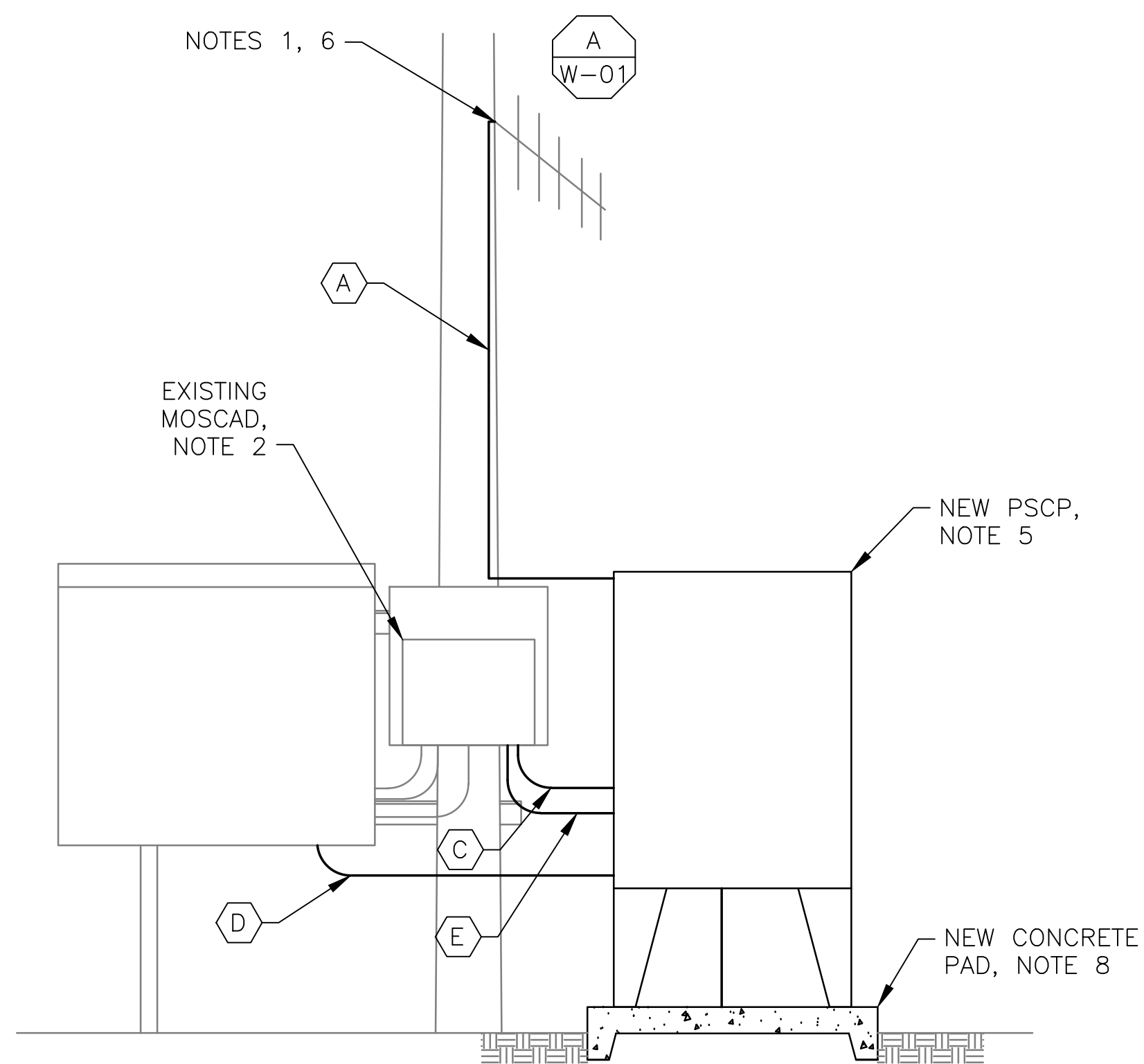
3 NEW SCADA PANEL INSTALLATION SCALE: NOT TO SCALE
