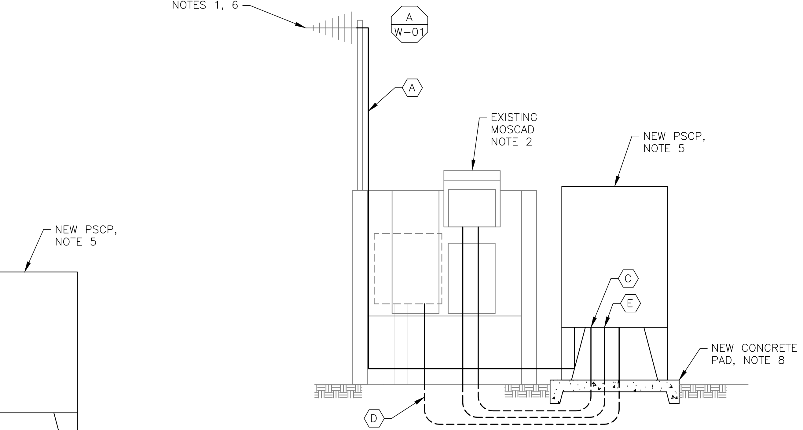
3 NEW SCADA PANEL INSTALLATION SCALE: NOT TO SCALE
